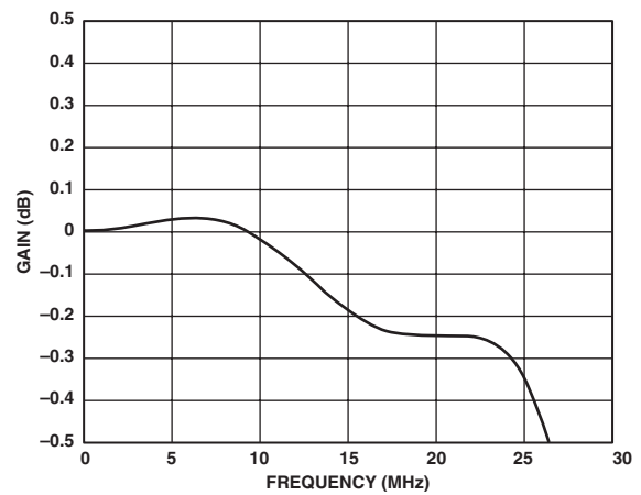
Figure 28. HD Sinc Filter Disabled
